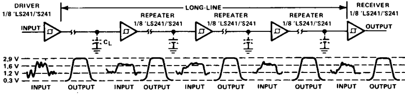
'LS241, 'S241 USED AS REPEATER/LEVEL RESTORER
