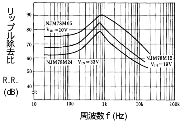
NJM78M05/12/24 リプル除去比特性例 ( I_o = 350\text{mA} , e_{in} = 1V_{P-P} , T_j = 25 )
