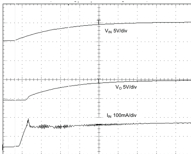
Figure 22. Startup Waveforms
