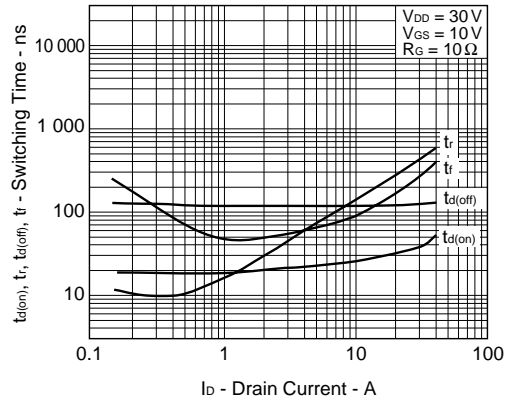
SWITCHING CHARACTERISTICS
