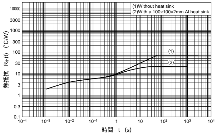
R_{th(t)} - t
